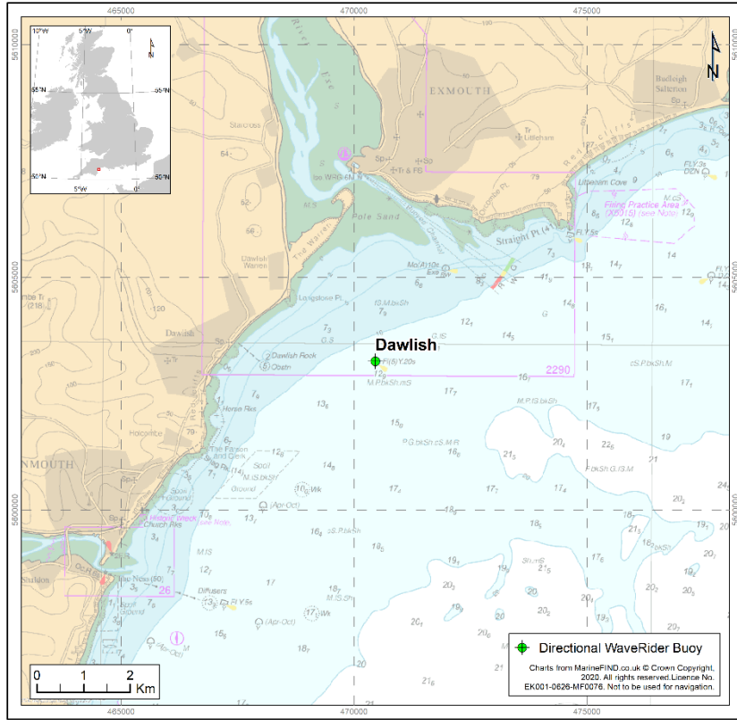
Figure 1: Dawlish Wave Buoy
