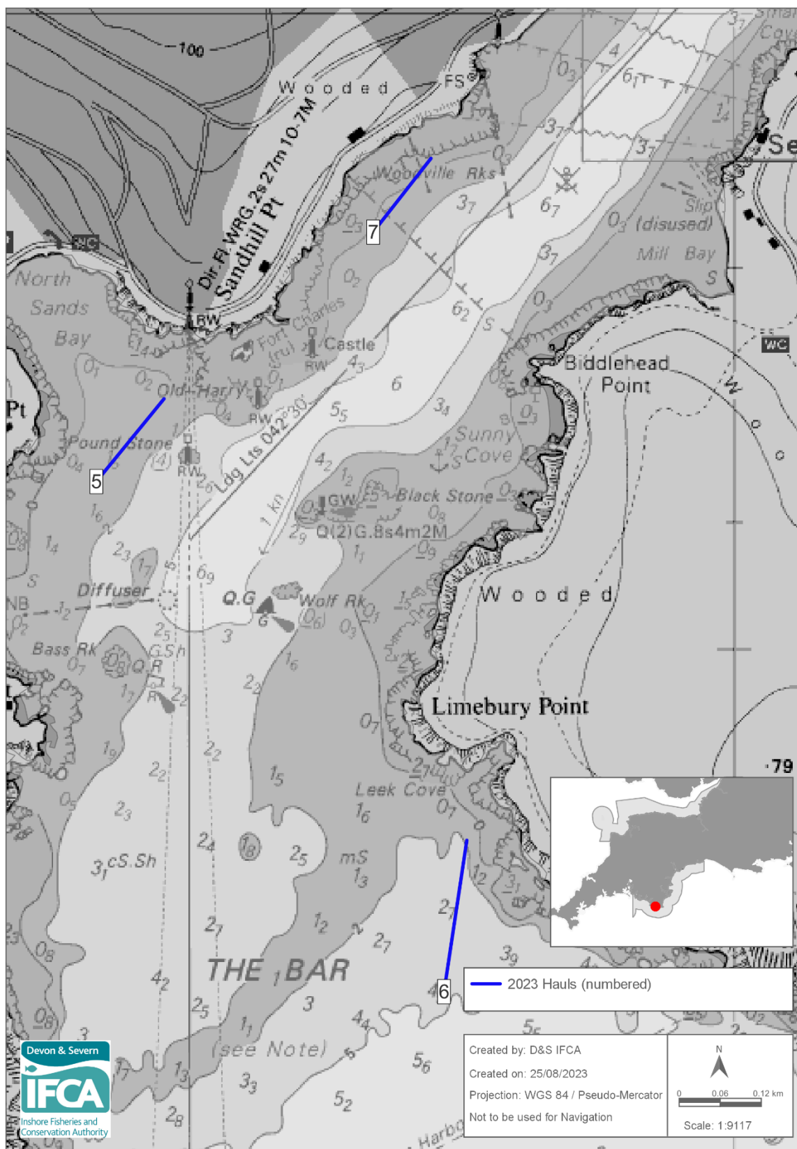
Figure 3. Sequentially numbered hauls of gillnets conducted in January 2023, showing hauls conducted south of a line between Snapes Point and Scoble Point (hauls 5 – 7).
