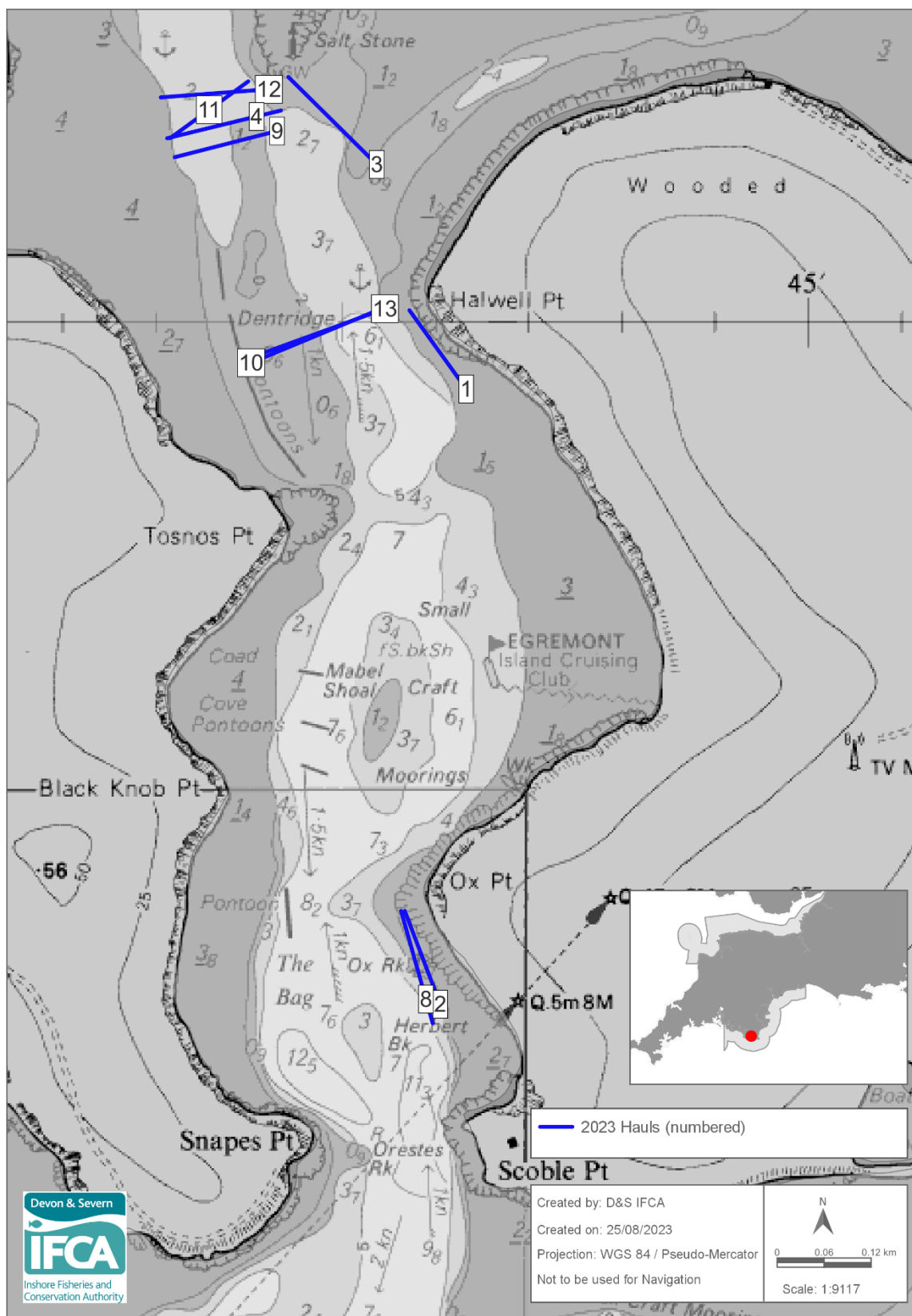
Figure 2. Sequentially numbered hauls of gillnets conducted in January 2023, showing hauls conducted north of a line between Snapes Point and Scoble Point (hauls 1 – 4 and 8 – 13).
